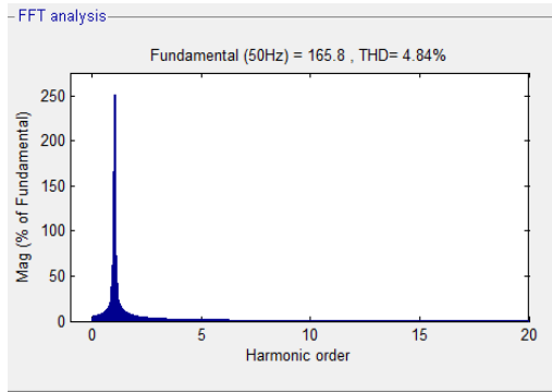
Fig6FFTanalysisofcascadedmultilevelinverter
