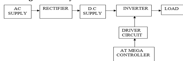
Figure 2. Block diagram of a multilevel inverter
