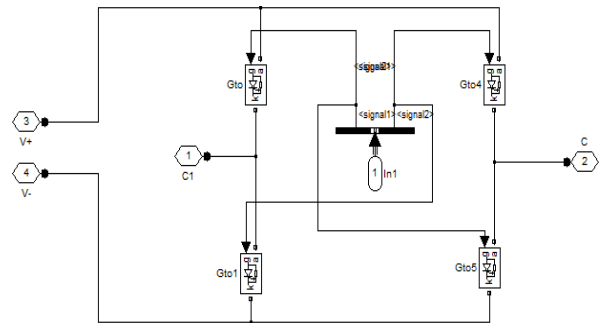
Figure 4 sub-system A1 block of 7 level h-bridge inverter
