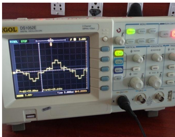
Figure8DSOOutput
