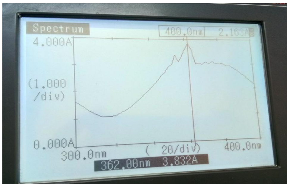
(Fig. 1. Identification Curve of Furazolidone)
