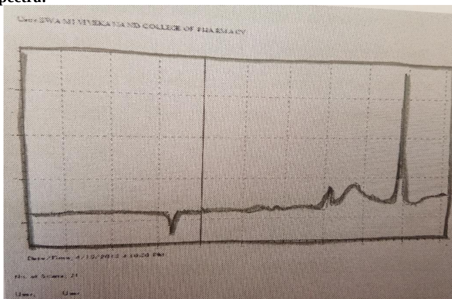
(Fig. 3. IR Spectra of Furazolidone)
