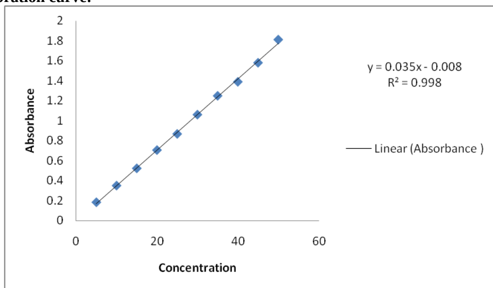
(Fig. 2. Calibration Curve of Furazolidone)
