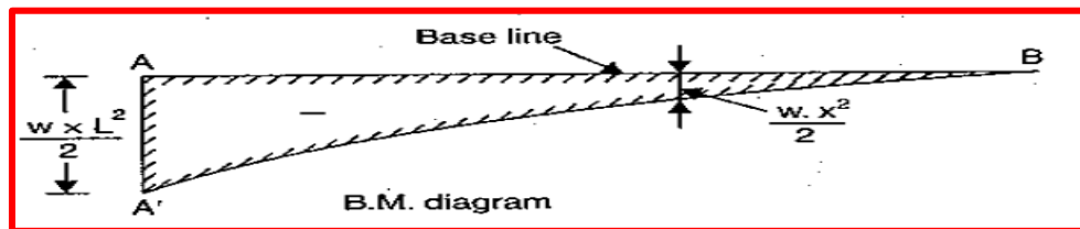
Fig 3.2: Bending moment diagram for sweep rake
