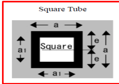
Fig 3.3: Square cross-section of a sweep rake
