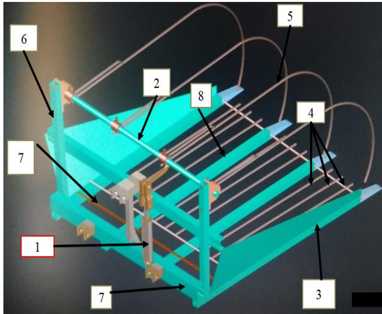
Fig 3.4: Different components of the developed device
